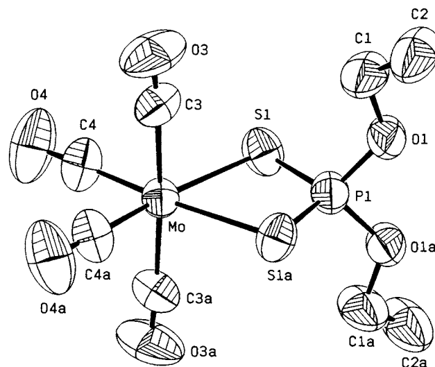
Fig. 1. ORTEP diagram of the anionic complex [Mo(CO)_4\{\eta^2-S_2P(OEt)_2\}]^- ( 1 ).
